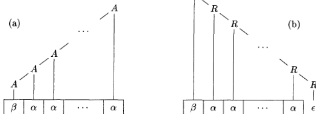
Left- and right-recursive ways of generating a string
